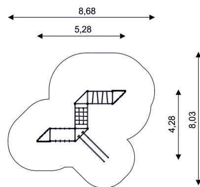
Minimal space
